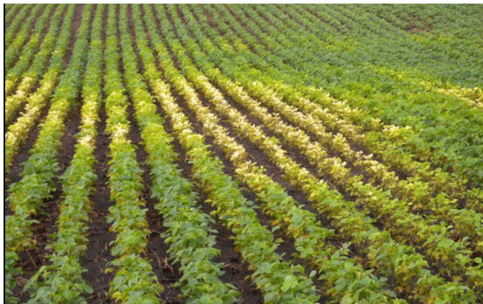
Figure 6. HPPD (Group 27) corn herbicide carryover to soybean.
